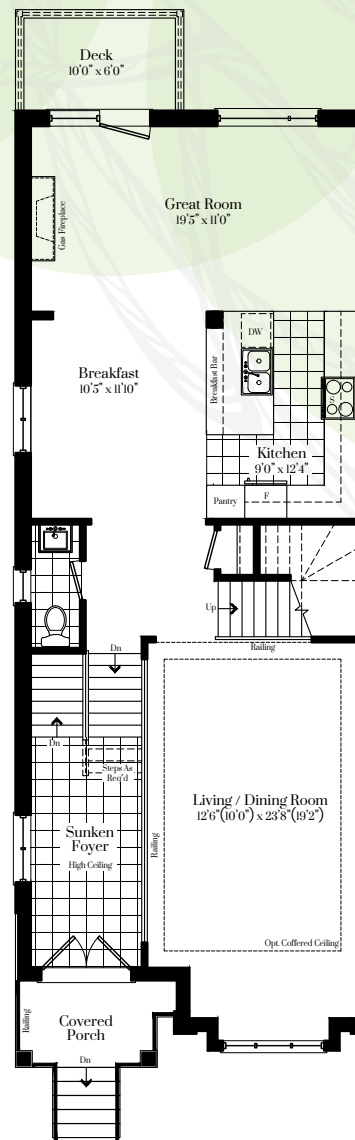
MAIN FLOOR
